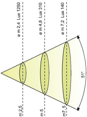
Standard Optics
